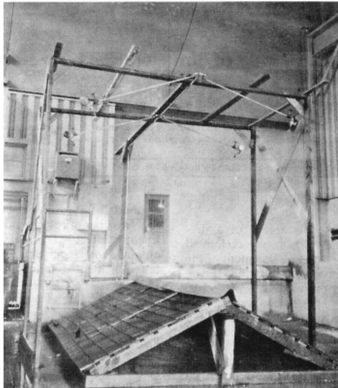
Figure 1. Rain test apparatus suitable for Method A (from ASTM D 2898-94).
