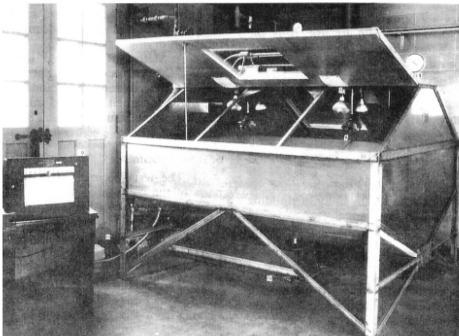
Figure 2. Exposure chamber suitable for Method B (from ASTM D 2898-94).
